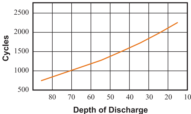
Cycle Life - Series 4000
