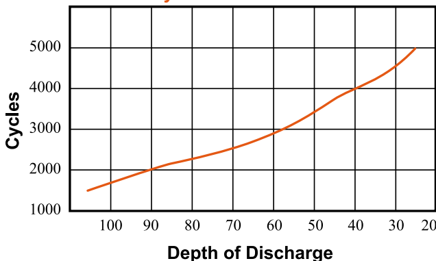
Cycle Life - Series 5000
